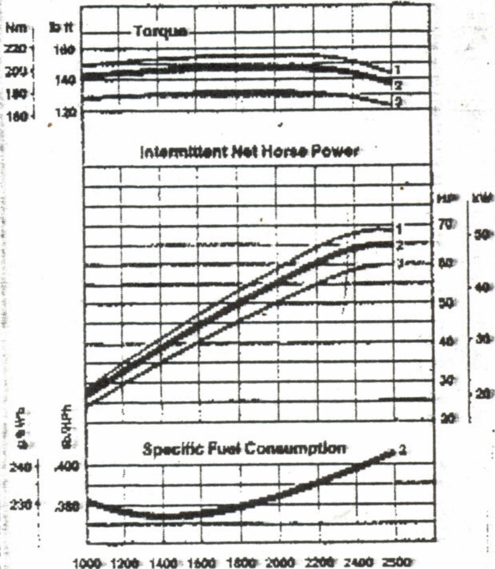
Performance Chart D-208 2500 RPM
