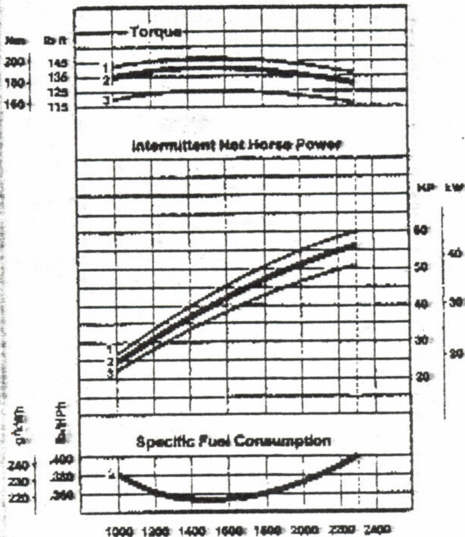
Performance Chart D-206 2300 RPM
